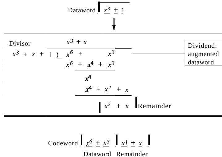
Figure 10.22 CRC division using polynomials
