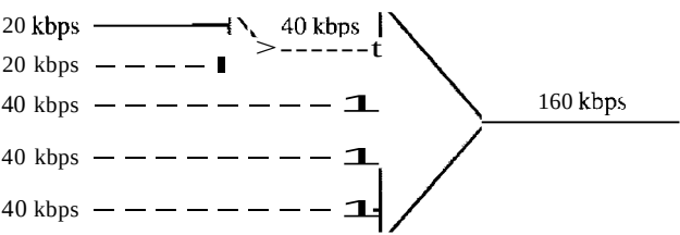
Figure 6.19 Multilevel multiplexing
